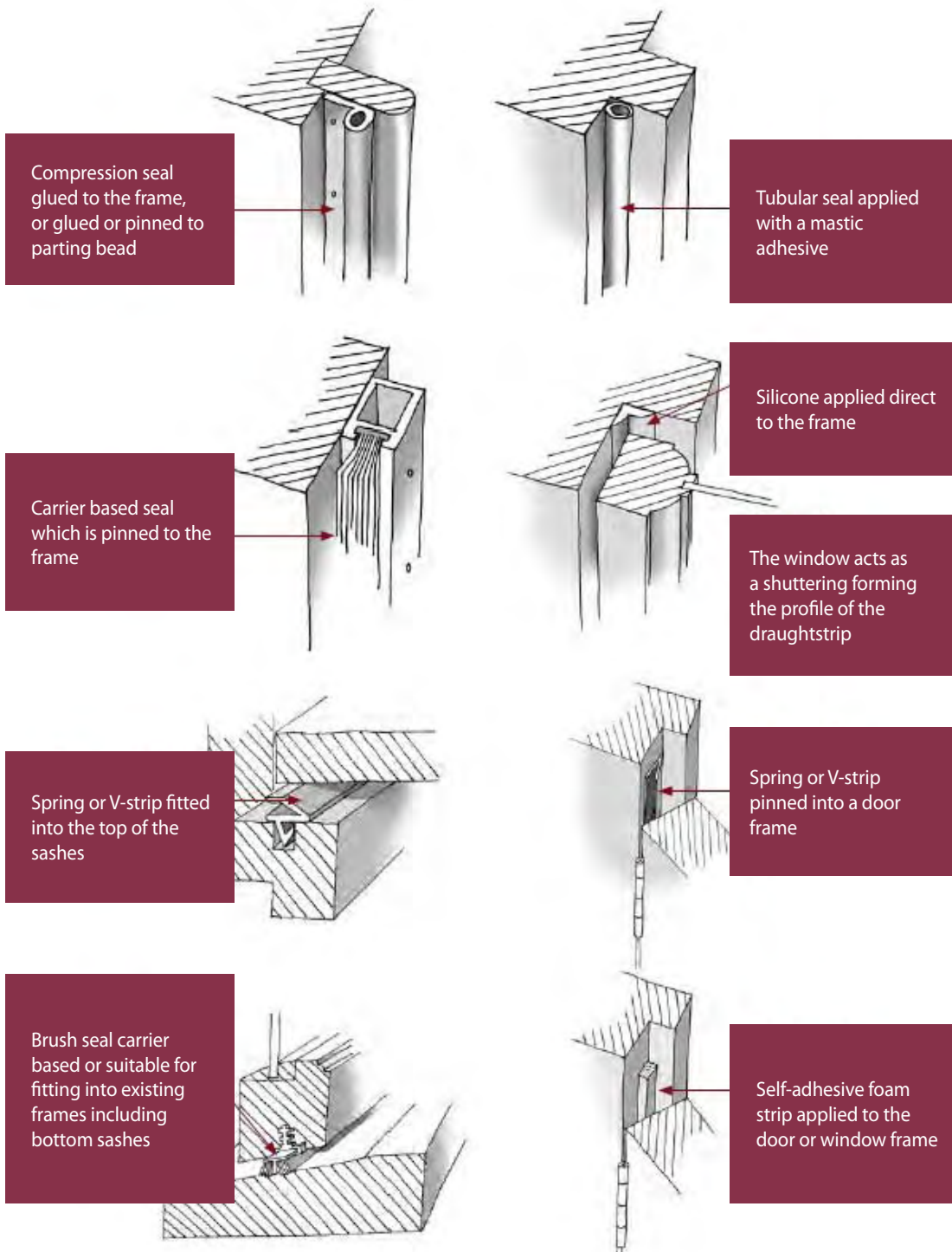
Examples of draught-proofing products for different junctions (drawing courtesy of Changeworks)
